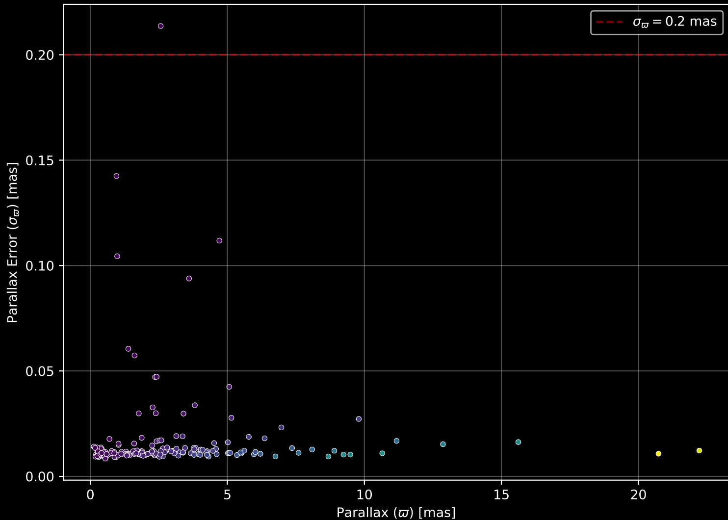
APOGEE DR17 Field: [290-28-O_TESS] Parallax Quality (n= 180)
