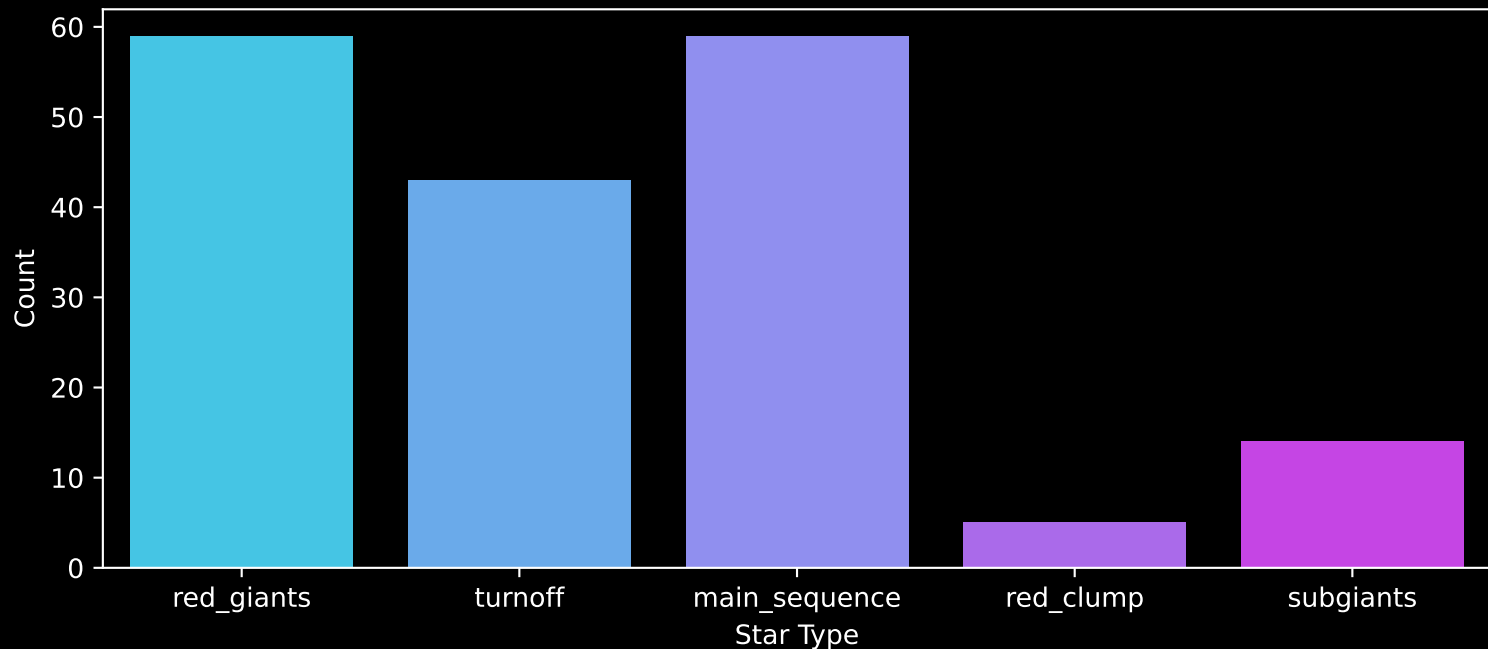
APOGEE DR17 Field: [290-28-O_TESS] Count plot of Star Type
