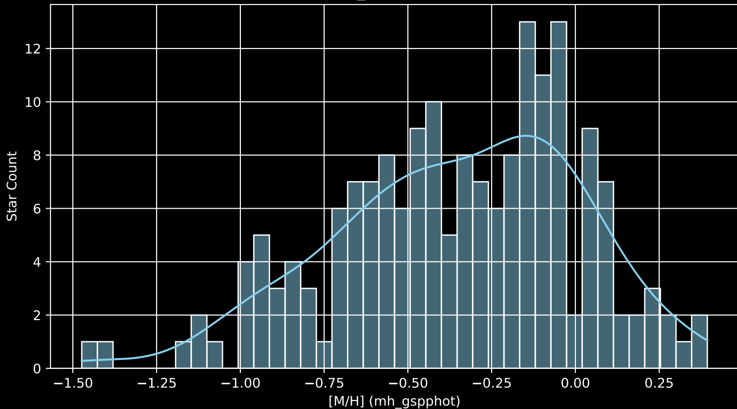
APOGEE DR17 Field: [290-28-O_TESS [M/H] (mh_gspphot) (n= 180)
