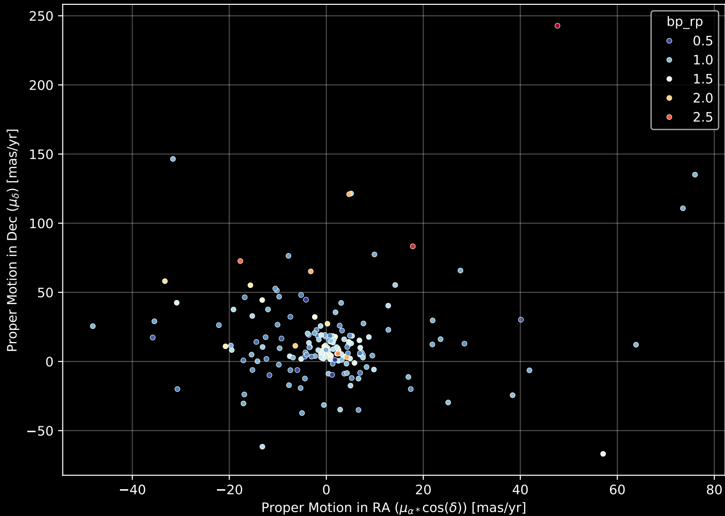
APOGEE DR17 Field: [290-28-O_TESS] Proper Motion Diagram (n= 180)
