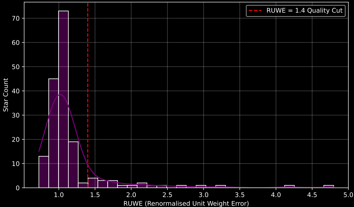
GAPOGEE DR17 Field [290-28-O_TESS] RUWE Distribution (n= 173)
